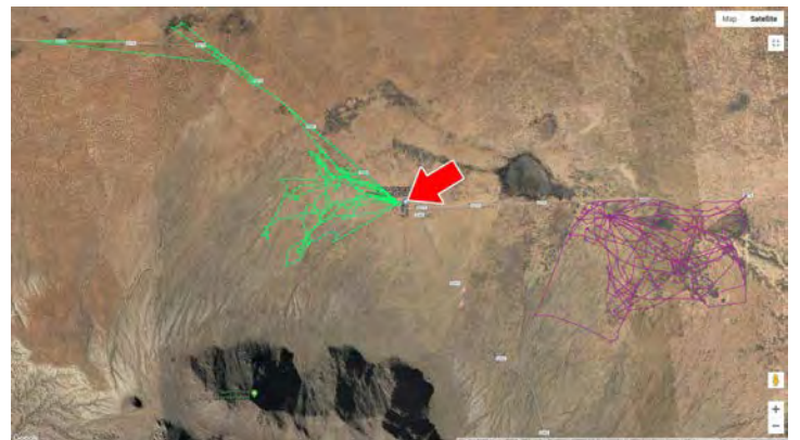
Real-time GPS locations of two cows (green and purple polygons above) grazing large desert pastures at the NMSU Chihuahuan Desert Livestock Research Center during preliminary tests in June 2019. Data are available via the Abeeway™ dashboard online. The system recorded approximately 77% of GPS fixes (10 min intervals). The antenna and gateway (red arrow) were located about 4 km from the farthest GPS point recorded.
